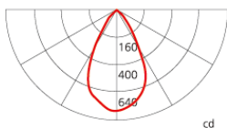
LMR16-5 K30D60
