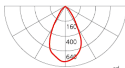
LMR16-5 K30D60
